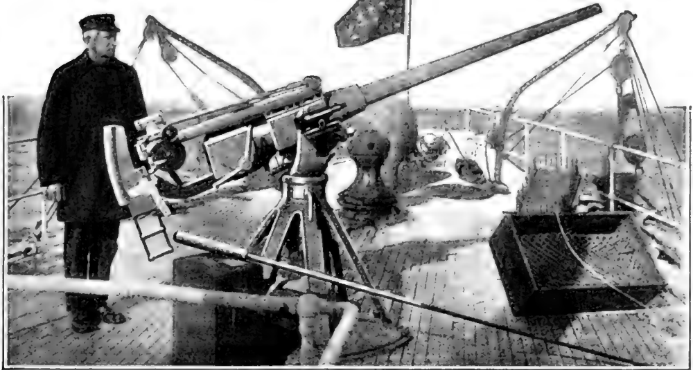
In Line Shooting with the Rapid-Fire Guns a Projectile About Six Feet Long Is Used. The End Which Is Inserted in the Gun Is a Cylindrical Piece of Steel Slightly Smaller Than the Bore of the Gun. The Line Is a Hemp Rope About the Size of a Wash Line
